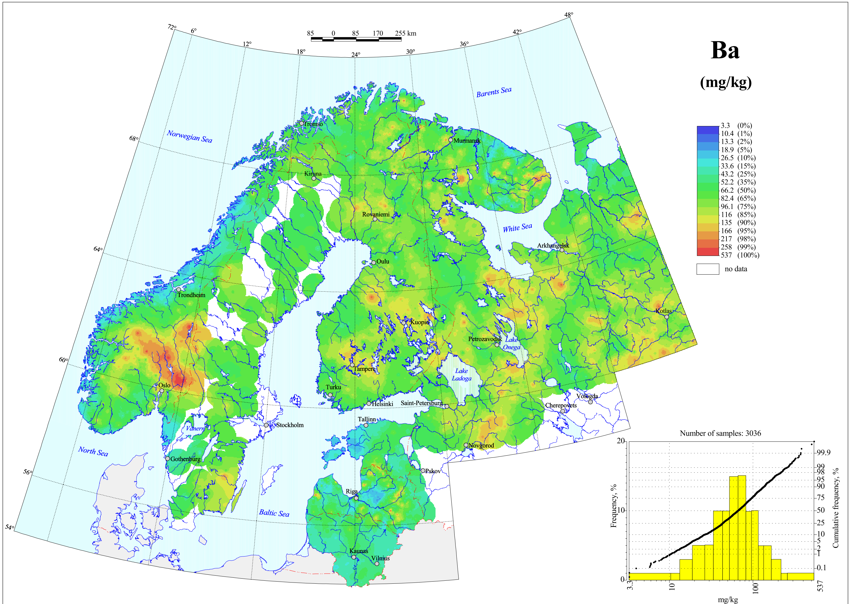
Barium in Organic Soil Layer, Total Content
